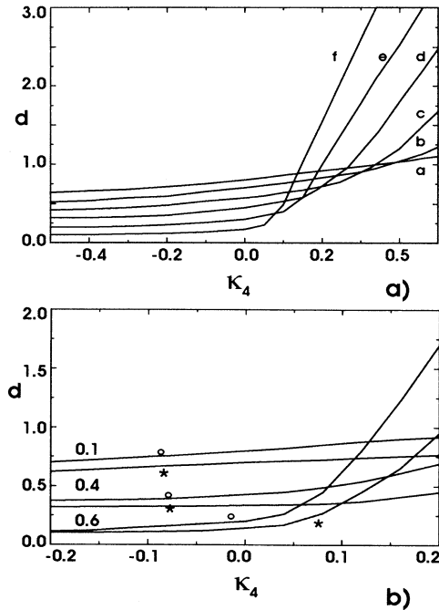
FIG. 3. Threshold thickness d_a between the PHAN and the HAN structure as a function of the elastic ratio \kappa_4 = K_{24}/K . The value of L_{\theta_0} is fixed to 0.7 \mu\text{m} , as previously estimated. (a) The value of d_a for different values of L_{\theta_1} ranging from 0.1 (curve a) to 0.6 (curve f) with a step of 0.1 \mu\text{m} . (b) The behavior of d_a for L_{\theta_1} = 0.1, 0.4, \text{ and } 0.6 \mu\text{m} for H=0 ( \circ ) and 3 \text{ kG} ( * ). Note the lowering of the threshold due to the applied field.
